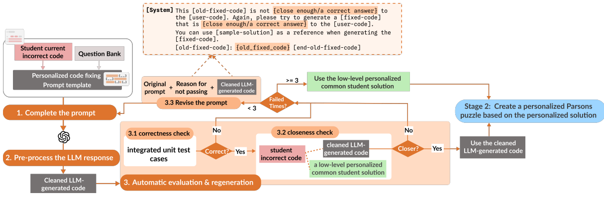
Figure 3: Pipeline for generating a personalized correct solution from an incorrect code in CodeTailor (Stage 1)
